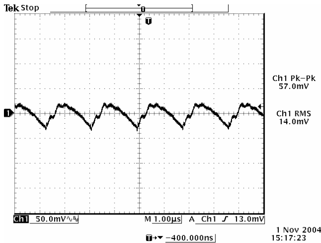
Ripple and noise at full load, V_{in}=5\text{ V} , V_o=12\text{ V}
